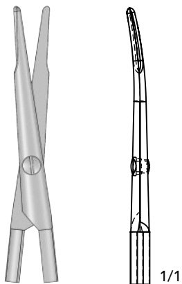
Tenotomy 4 ½" (115 mm)
